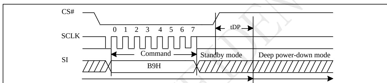
Figure 10-30 Deep Power-down (DP) Sequence (Command B9)
